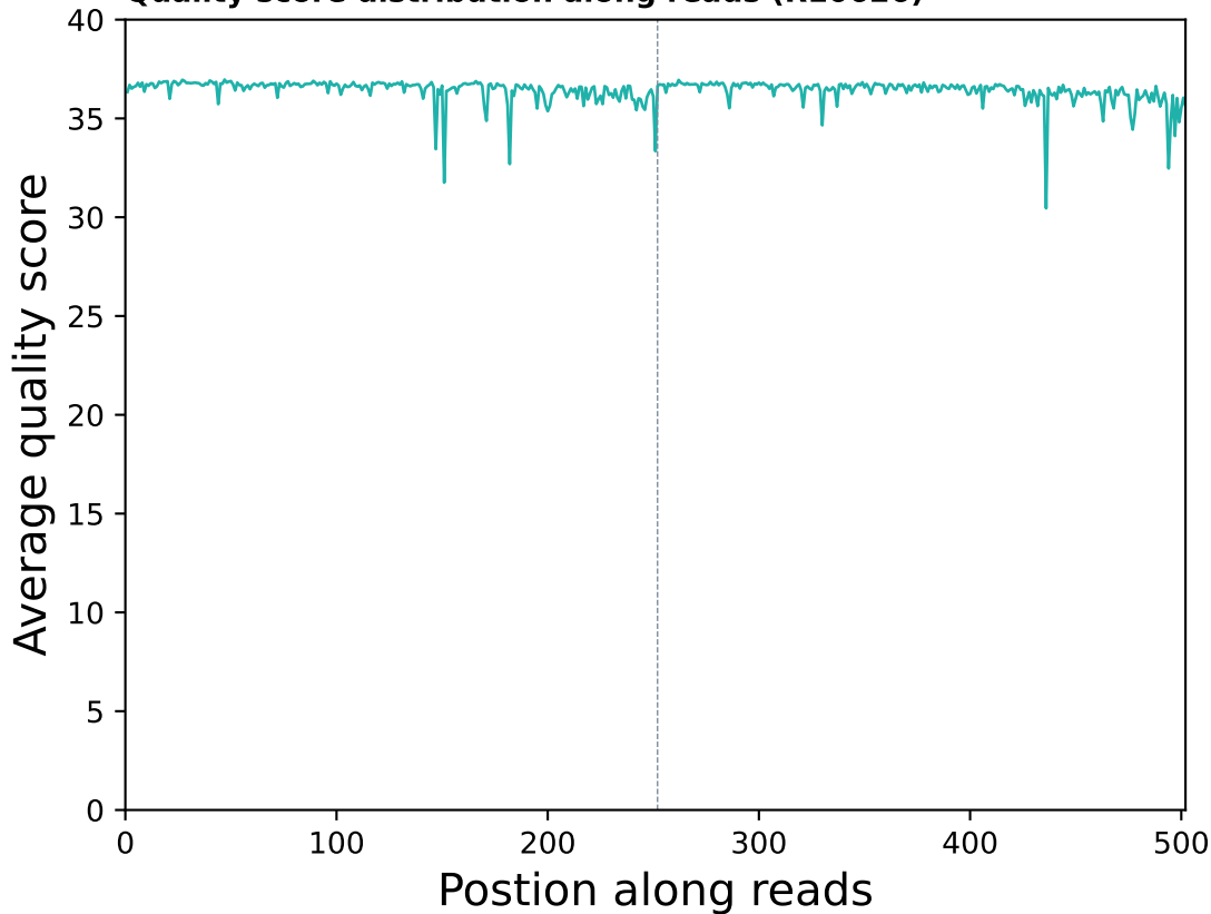
Quality score distribution along reads (R10626)
